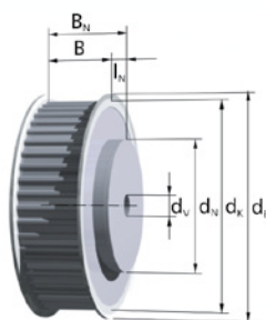
Stock pulleys over z = 24 with flanges
