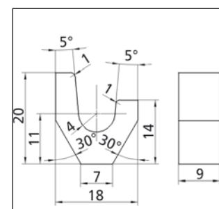
Profile No. 2.3.2.018.020
