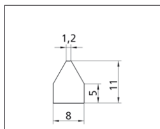
Depth: 10 mm Profile No. 2.3.3.008.011
