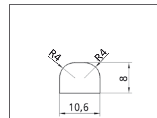
Depth: 100 mm Profile No. 2.3.2.008.010
