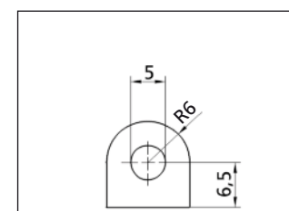
Depth: 100 mm Profile No. 2.3.2.010.020
