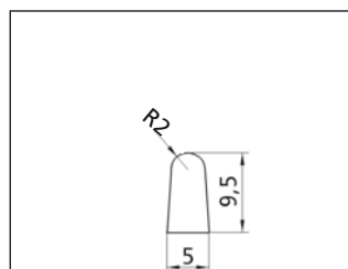
Depth: free Profile No. 2.3.3.009.005
