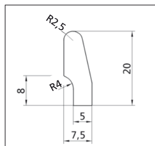
Depth: 70 mm Profile No. 2.3.3.007.020
