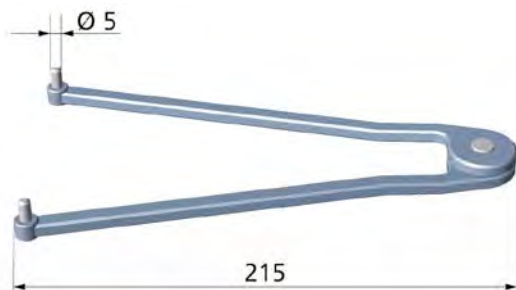
Stirnlochschlüssel, Typ 40 758
