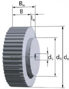
Stock pulleys up to z = 20 without flanges
