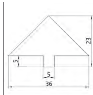
Depth: 100 mm Profile No. 2.3.3.023.036
