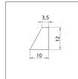
Depth: 130 mm Profile No. 2.3.2.010.012
