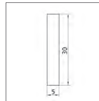
Depth: 100 mm Profile No. 2.3.2.030.005
