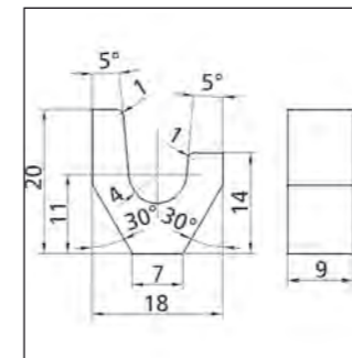
Profile No. 2.3.2.018.020
