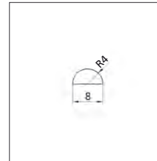
Depth: 100 mm Profile No. 2.3.1.008.004
