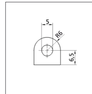
Depth: 50 mm Profile No. 2.3.2.012.012
