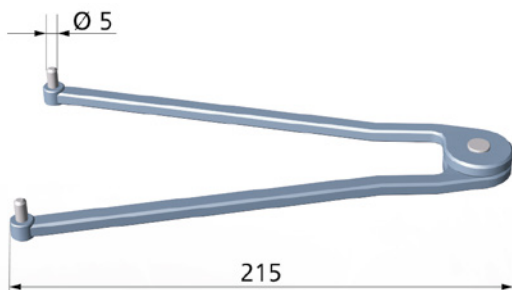
Stirnlochlüssel, Typ 40 758
